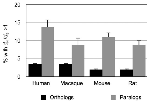
Figure 2. Positive selection on gene duplicates. The proportion of lineage-specific subtrees and orthologs with evidence for positive selection using a likelihood ratio test between models M1a and M2a ( P < 0.05 ). Standard errors are shown.
